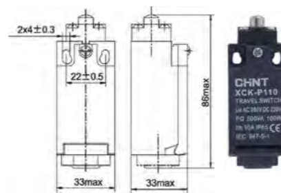
YBLX-CK-P110 Travel Switch YBLX-CK/P110 R349.24
