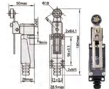
YBLX-ME/8108 Travel Switch Adjustable Roller Rotating Rod R256.38
